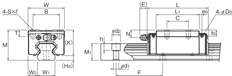
HSR15~35R/LR/RM/LRM型
