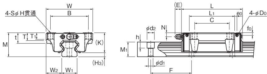
HSR15~35C/LC/CM/LCM型
