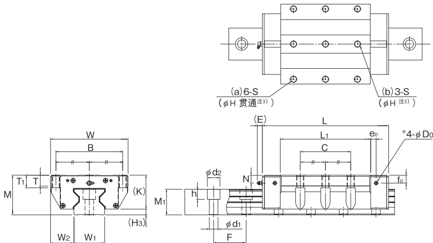
SRG100LC形
