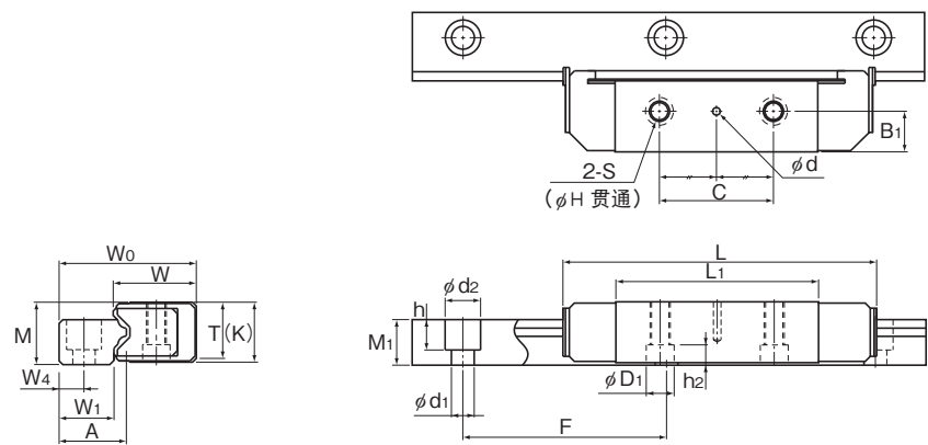
HR1123~2555M/T/TM型
