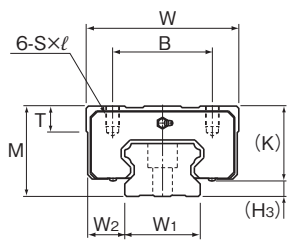
HSR100~150HR型
